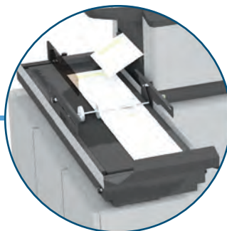
High-Capacity Output Conveyor Holds filled envelopes, can be used straight-on or at 90°
