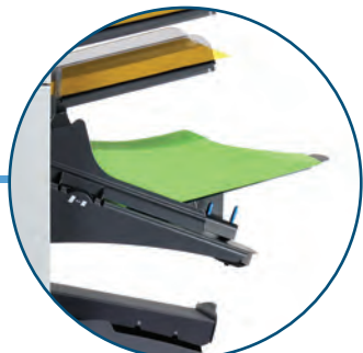
Optional Production Feeder Holds up to 325 BRENs or 1,200 inserts up to 6" long
